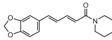
Piperine
