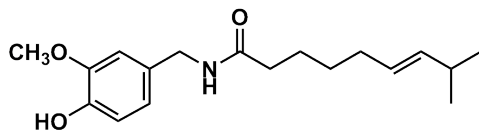
Capsaicin
