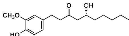
6-Gingerol
